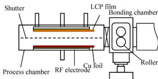
Figure 2 Schematic diagram for a SAB tool.
